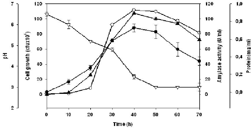
Figure 1: Time course of growth (○), pH (▽), amylase (▲) and soluble protein (●) production by Lactobacillus fermentum 04BBA19 in 1% (w/w) soluble starch medium at 40°C, pH 6.0. The data shown are averages of triplicates assays within 10% of the mean value.
