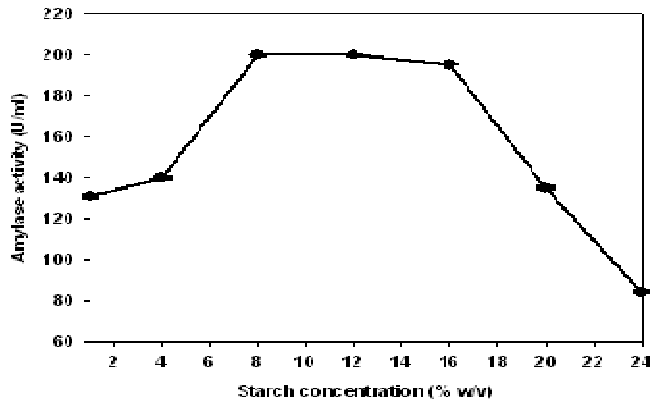
Figure 3: The effect of starch concentration on enzyme production by Lb. fermentum 04BBA19. The data shown are averages of triplicate assays with SD within 10% of mean value.
