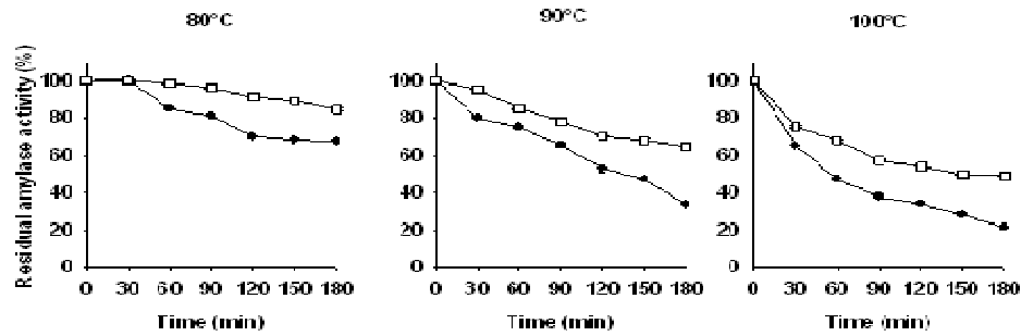
Figure 7: Thermostability pattern of \alpha -amylase from Lb. fermentum 04BBA19, at 80, 90, 100°C without \text{CaCl}_2 \cdot 2\text{H}_2\text{O} (●) and with 0.1% w/v \text{CaCl}_2 \cdot 2\text{H}_2\text{O} (□) at different temperatures (80, 90, 100°C). The enzyme was pre-incubated at optimum pH, for 30, 60, 90, 120 and 180 min at temperatures (80-100°C). The remaining activity was determined incubating the enzyme at optimum temperature, 60°C for 30 min. The data shown are averages of triplicate assays with SD within 10% of mean value.
