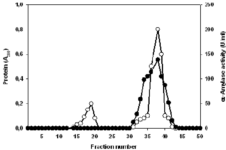
Figure 4: Elution pattern of starch column chromatograph (φ1,5x15cm), of Lb. fermentum 04BBA19 α-amylase; absorbance at 280 nm (○), α-amylase activity (●). Column (φ 1.5x15 cm) was washed with 0.25 M NaCl to remove impurities; α-amylase from Lb. fermentum 04BBA19 was eluted with 0.05 M Na 2 CO 3 at the flow rate of 3ml/20 min.
