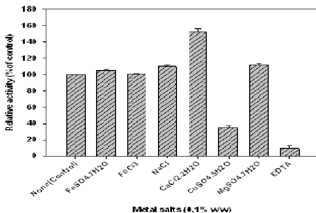
Figure 9: Effect of metal salts and EDTA on the activity of \alpha -amylase from Lb. fermentum 04BBA19. The data shown are averages of triplicate assays with SD within 10% of mean value.
