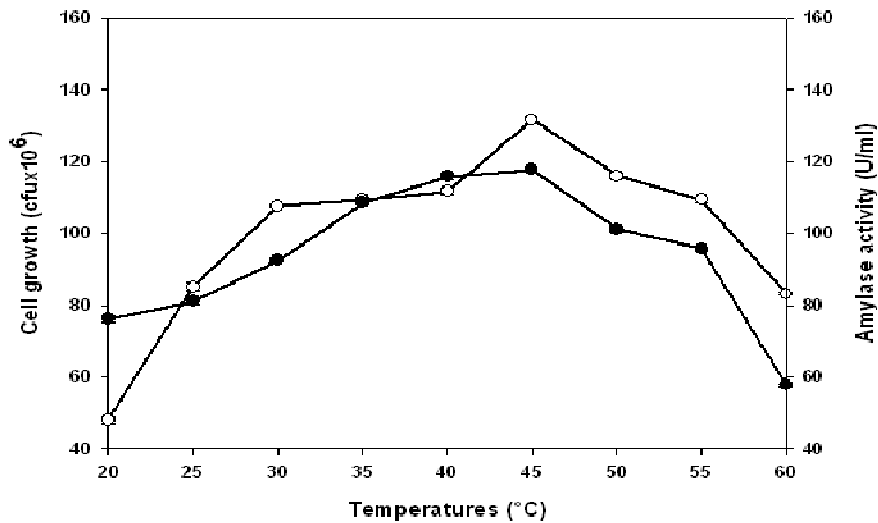
Figure 2: Effect of temperature on growth (○) and \alpha -amylase production by Lb. fermentum 04BBA19 grown in 1% (w/w) soluble starch medium, pH 6.0. The data shown are averages of triplicate assays with SD within 10% of mean value.
