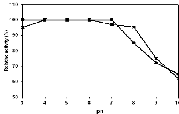
Figure 8: Effect of pH on the activity (x) and stability (■) of Lb. fermentum 04BBA19 \alpha -amylase. The data shown are averages of triplicate assays with SD within 10% of mean value.
