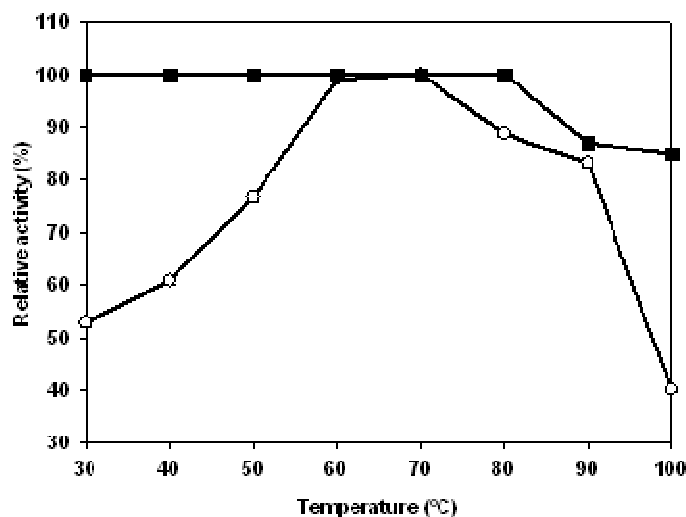
Figure 6: Effect of temperature on the activity (○) and thermal stability (■) of Lb. fermentum 04BBA19 \alpha -amylase. The reaction mixture contained 5 ml substrate (1% w/v soluble starch in 100 mM; phosphate buffer, pH 6.0) and 0.5 ml partial purified enzyme solution. The mixture was incubated for 30 min at various temperatures (30-100°C) under standard enzyme assay condition. The enzyme displayed maximal activity at (60-70°C). For determination of the thermostability of amylase, the enzyme was pre-incubated at optimum pH, for 30 min at temperatures range of 30-100°C. The remaining activity was determined incubating the enzyme at optimum temperature, 60°C for 30 min. The data shown are averages of triplicate assays with SD within 10% of mean value.
