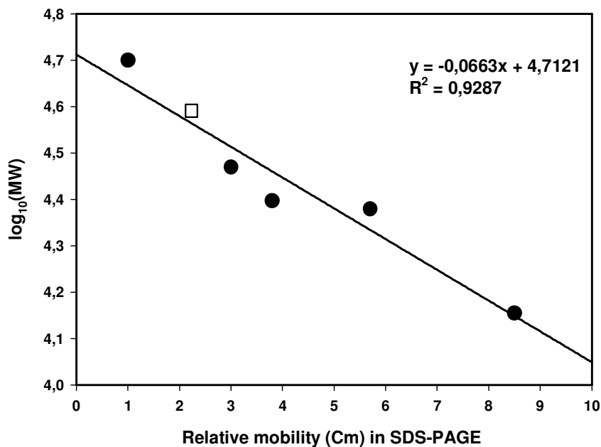
Figure 5: Determination of relative molecular weight of α-amylase from Lb fermentum 04BBA19 in SDS-PAGE electrophoresis, (●): standard proteins, (□):α-amylase from Lb fermentum 04BBA19
